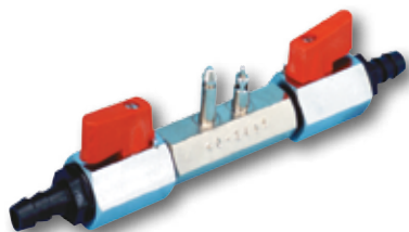
2-way fuel valves for hose Ø 10 mm.
