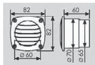
Ventilation Shaft with Gasket
