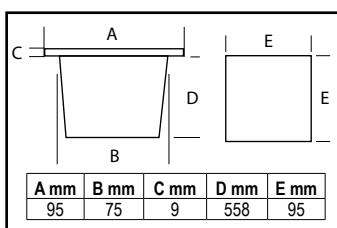
Tap in a box with lead (only cold water)
